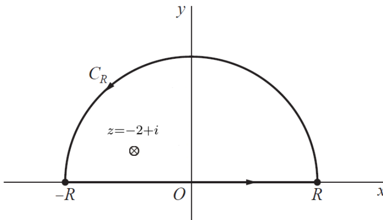
Figure 1: This is Fig. 99 with the singularity at z = -2 + i marked.
